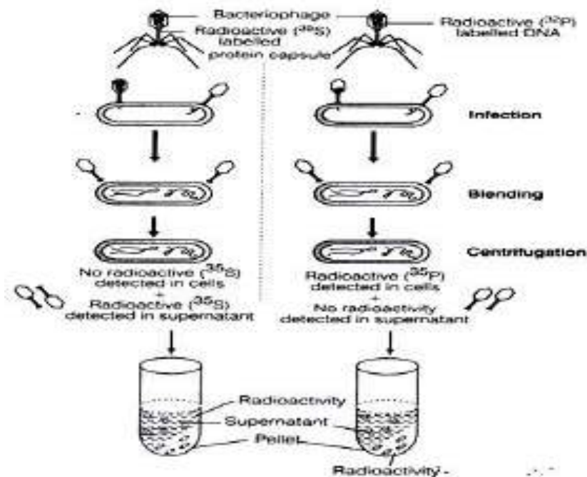
Fig. 8.5 Hershey and Chase experiment
